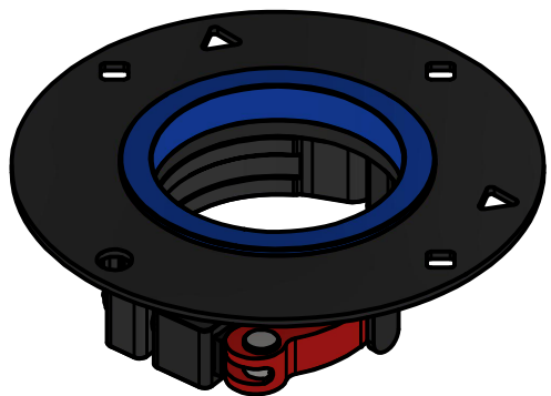
QTY: (1) SECONDARY GUY RING-350 P/N: BSM3-A-M100-RNG-CL0 1.51 lbs / 0.69 kg
