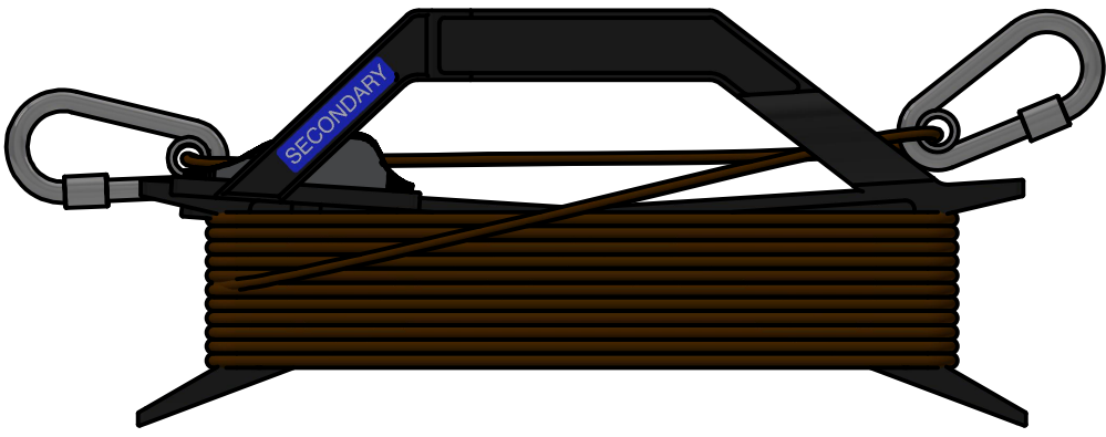
QTY: (4) 350G HEAVY GUY ROPE W/CLEAT-18M-SECONDARY P/N: 350G-P-GC18-2ND-BLU 1.54 lbs / 0.70 kg (each)
