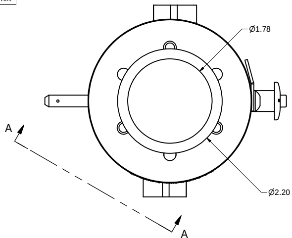
OVERHEAD VIEW
