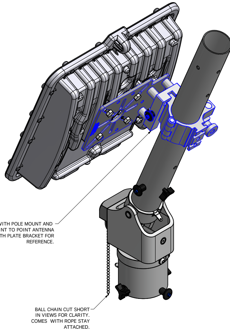
REFERENCE VIEW LANYARD NOT SHOWN FOR CLARITY
