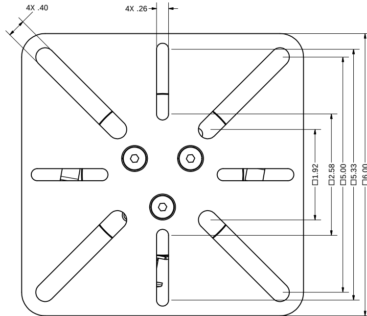
OVERHEAD VIEW
