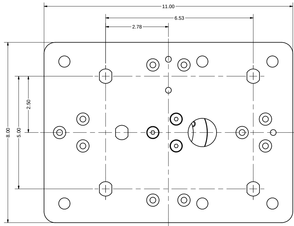
OVERHEAD VIEW
