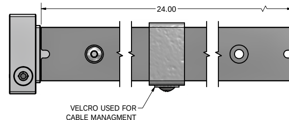
BSMU-P-A324-ARM-15S SIDE ARM-UNIVERSAL-1.5 X 24, WITH STRAIGHT BRACKET
