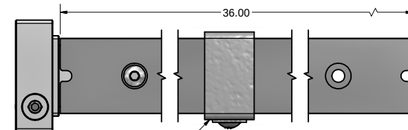
BSMU-P-A336-ARM-15S SIDE ARM-UNIVERSAL-1.5 X 36, WITH STRAIGHT BRACKET
