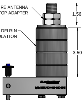
BSMU-K-M400-OE2-EM5 SIDE MOUNT-150 ARM-OE254 & COM201 ANTENNAS
