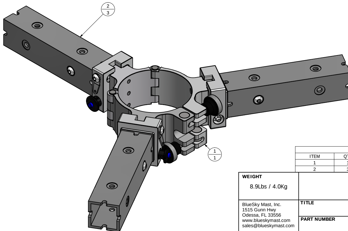
BSM3-P-A353-T00-000 POLE MOUNT-AL3-THREE WAY
