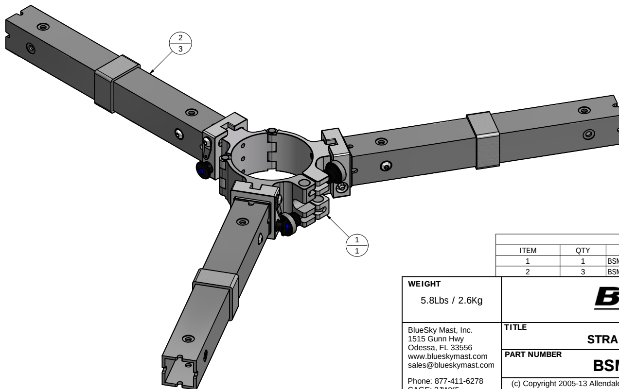
BSM3-P-A353-T00-000 POLE MOUNT-AL3-THREE WAY
