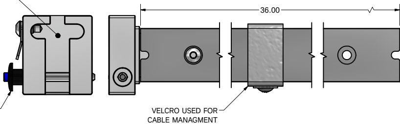
BSMU-P-A336-ARM-15S SIDE ARM-UNIVERSAL-1.5 X 36, WITH STRAIGHT BRACKET
