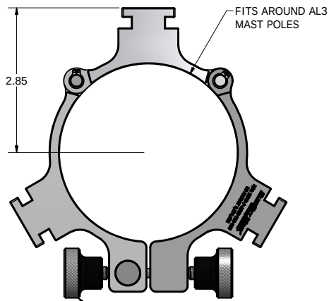
BSM3-P-A353-T00-000 POLE MOUNT-AL3-THREE WAY
