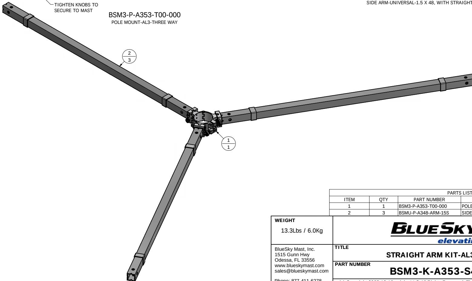
BSMU-P-A348-ARM-15S SIDE ARM-UNIVERSAL-1.5 X 48, WITH STRAIGHT BRACKET
