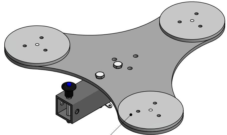
REFERENCE VIEW 7" LANYARD NOT SHOWN FOR CLARITY
