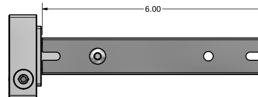
BSM2-P-A306-ARM-10S SIDE ARM-UNIVERSAL-1 X 6, WITH STRAIGHT BRACKET
