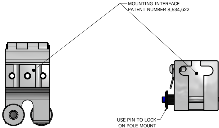
BSM2-P-A312-ARM-10S SIDE ARM-UNIVERSAL-1 X 12, WITH STRAIGHT BRACKET
