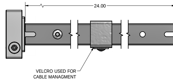
BSM2-P-A324-ARM-10S SIDE ARM-UNIVERSAL-1 X 24, WITH STRAIGHT BRACKET
