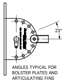
BSM2-K-A352-T44-BOL ARTICULATING ARM KIT-100 ARM-1 X 44 WITH BOLSTER PLATE, DUAL 7.8Lbs / 3.5Kg
