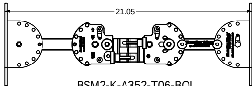
BSM2-K-A352-T06-BOL ARTICULATING ARM KIT-100 ARM-1 X 6 WITH BOLSTER PLATE, DUAL 4.6Lbs / 2.1Kg
