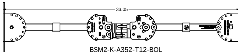
BSM2-K-A352-T12-BOL ARTICULATING ARM KIT-100 ARM-1 X 12 WITH BOLSTER PLATE, DUAL 5.2Lbs / 2.3Kg
