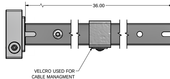
BSM2-P-A336-ARM-10S SIDE ARM-UNIVERSAL-1 X 36, WITH STRAIGHT BRACKET
