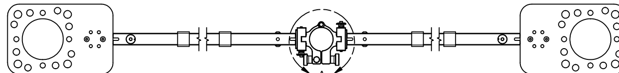
BSM2-K-A352-S44-NTO STRAIGHT ARM KIT-AL1/AL2-1 X44IN, DUAL NATO 7.4Lbs / 3.4Kg
