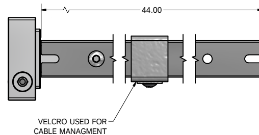
BSM2-P-A344-ARM-10S SIDE ARM-UNIVERSAL-1 X 44, WITH STRAIGHT BRACKET
