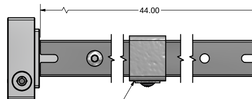
BSM2-P-A344-ARM-10S SIDE ARM-UNIVERSAL-1 X 44, WITH STRAIGHT BRACKET
