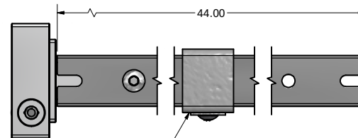
BSM2-P-A344-ARM-10S SIDE ARM-UNIVERSAL-1 X 44, WITH STRAIGHT BRACKET
