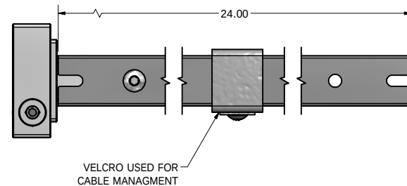
BSM2-P-A324-ARM-10S SIDE ARM-UNIVERSAL-1 X 24, WITH STRAIGHT BRACKET
