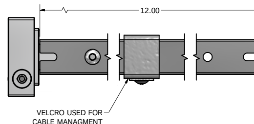
BSM2-P-A312-ARM-10S SIDE ARM-UNIVERSAL-1 X 12, WITH STRAIGHT BRACKET
