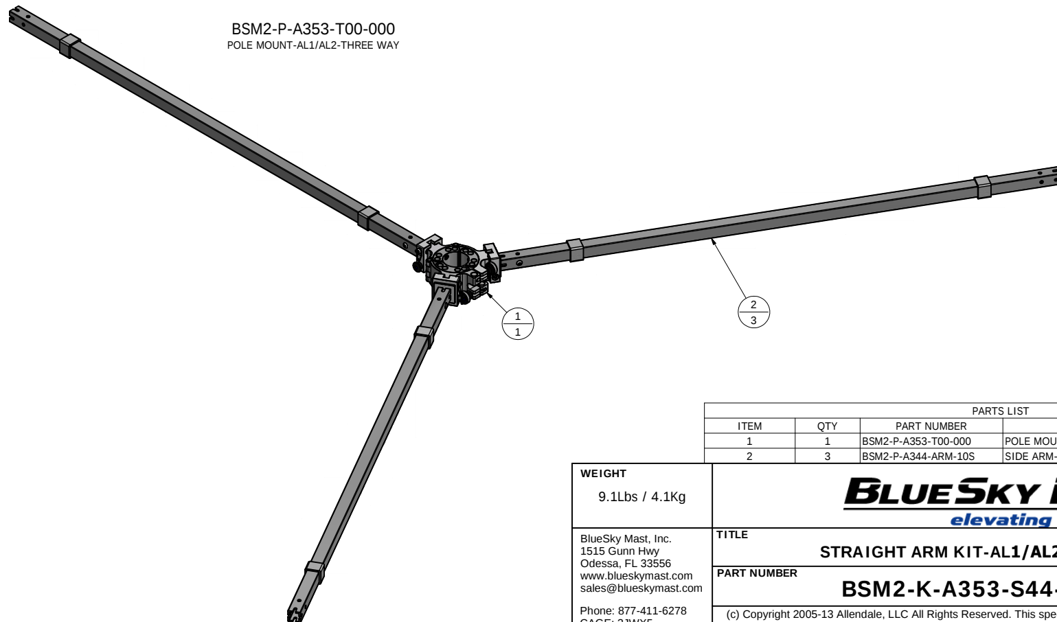
BSM2-P-A344-ARM-10S SIDE ARM-UNIVERSAL-1 X 44, WITH STRAIGHT BRACKET
