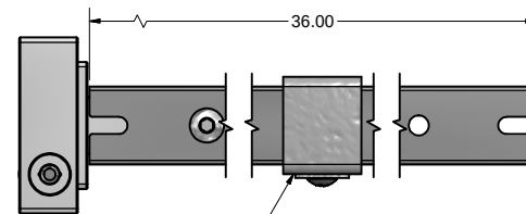
BSM2-P-A336-ARM-10S SIDE ARM-UNIVERSAL-1 X 36, WITH STRAIGHT BRACKET
