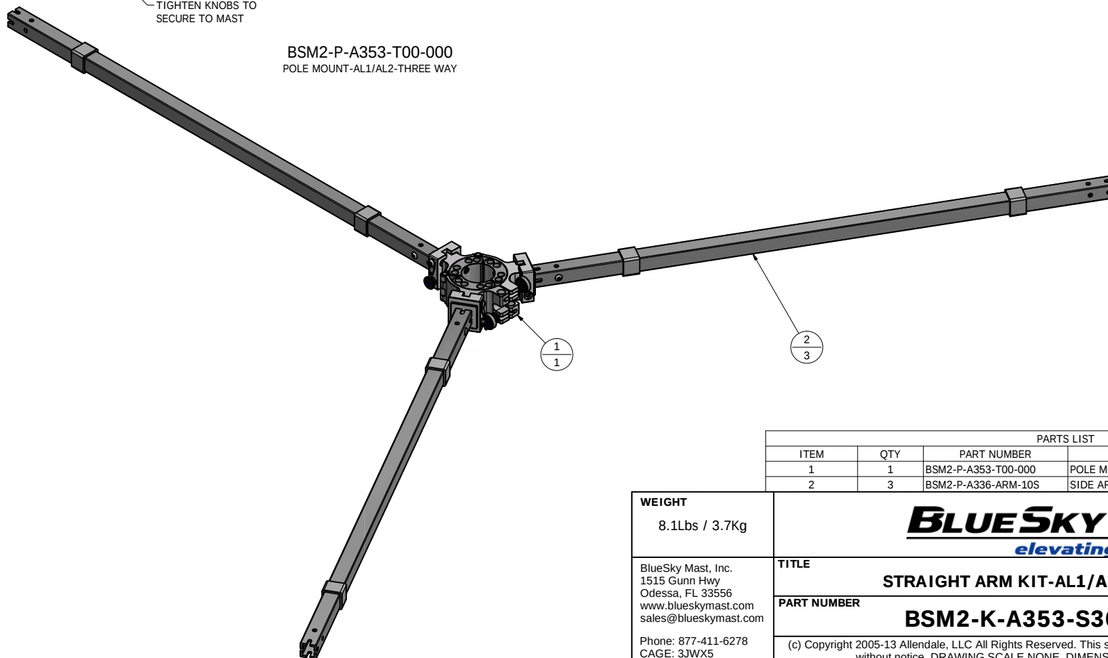
BSM2-P-A336-ARM-10S SIDE ARM-UNIVERSAL-1 X 36, WITH STRAIGHT BRACKET
