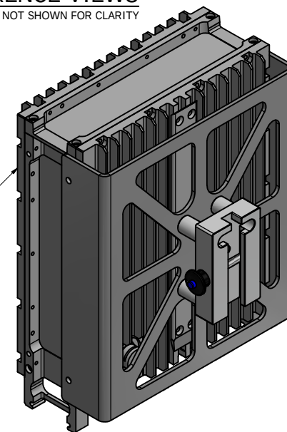
REFERENCE VIEWS 7" LANYARD NOT SHOWN FOR CLARITY
