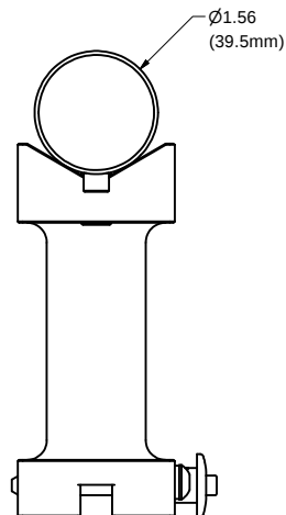
TOP VIEW AS COMMONLY PLACED
