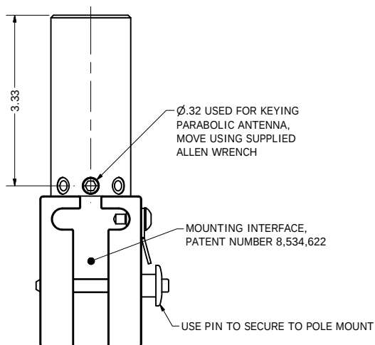
REAR VIEW AS COMMONLY PLACED LANYARD NOT SHOWN
