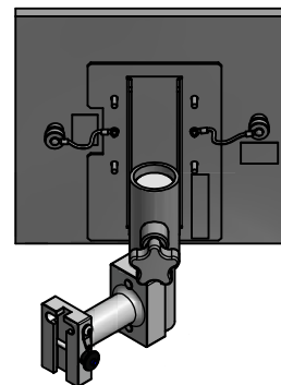
REFERENCE VIEWS 11.5 X 11.5 FLAT PANEL ANTENNA SHOWN 7" LANYARD NOT SHOWN FOR CLARITY
