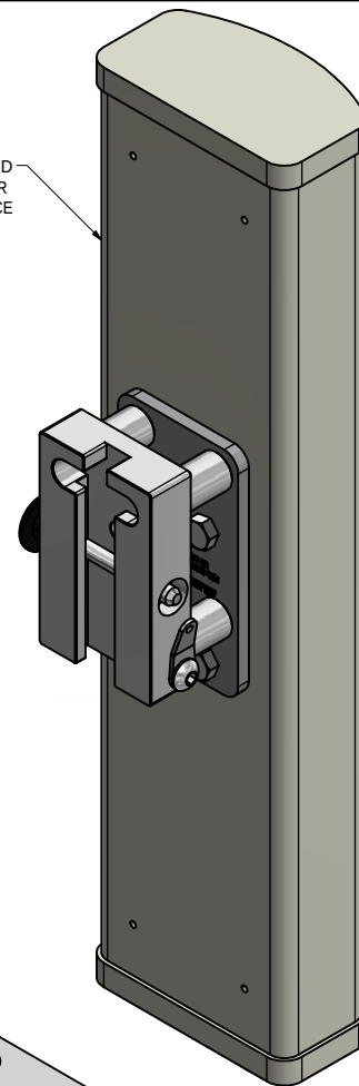
REFERENCE VIEWS 7" LANYARD NOT SHOWN FOR CLARITY
