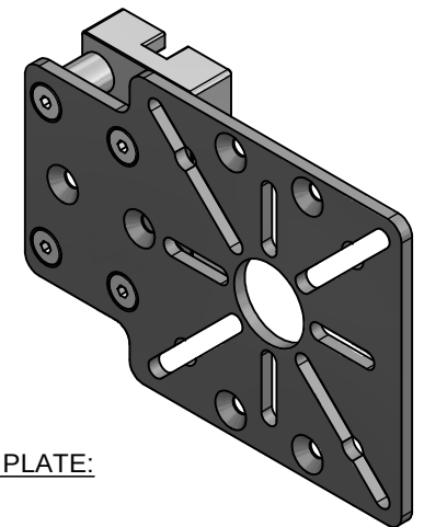
REFERENCE VIEWS 7" LANYARD NOT SHOWN FOR CLARITY
