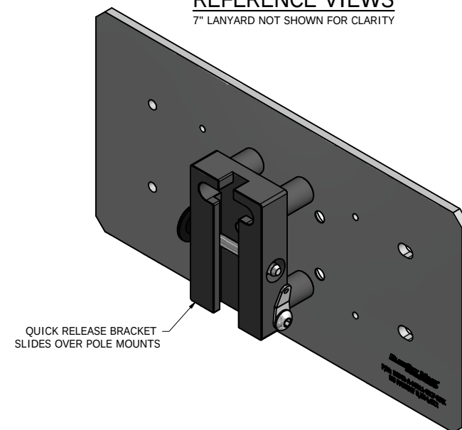
REFERENCE VIEWS
