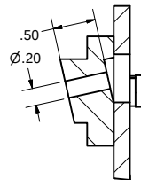
DETAIL B 4 PLACES
