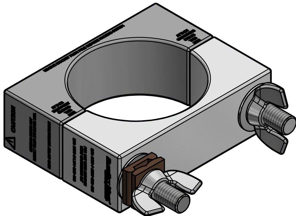
BST3-P-B205-GND-000 GROUNDING-AL3-BRACKET QTY 1
