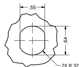
DETAIL A 2 PLACES
