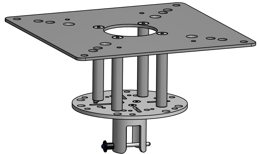
REFERENCE VIEW 7" LANYARD NOT SHOWN FOR CLARITY
