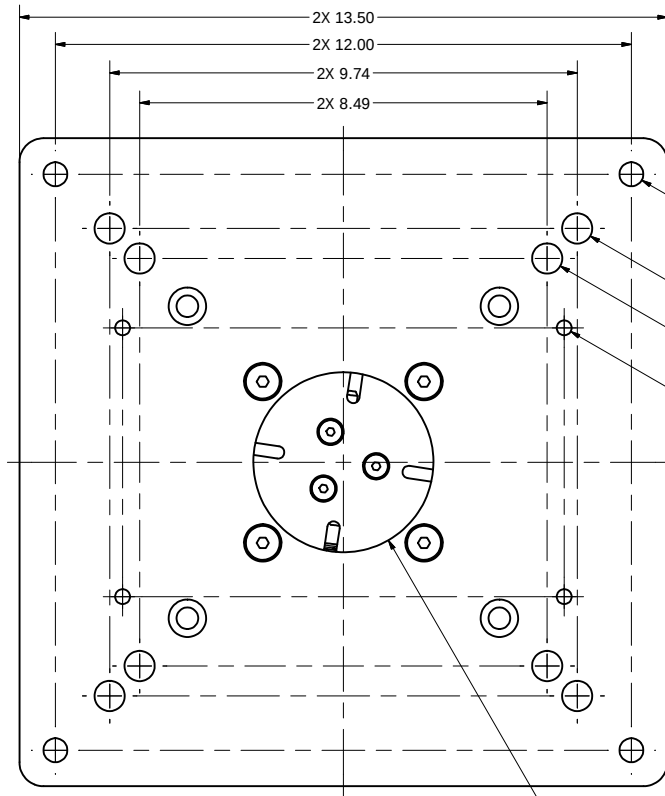
OVERHEAD VIEW
