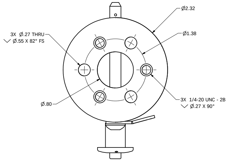
OVERHEAD VIEW
