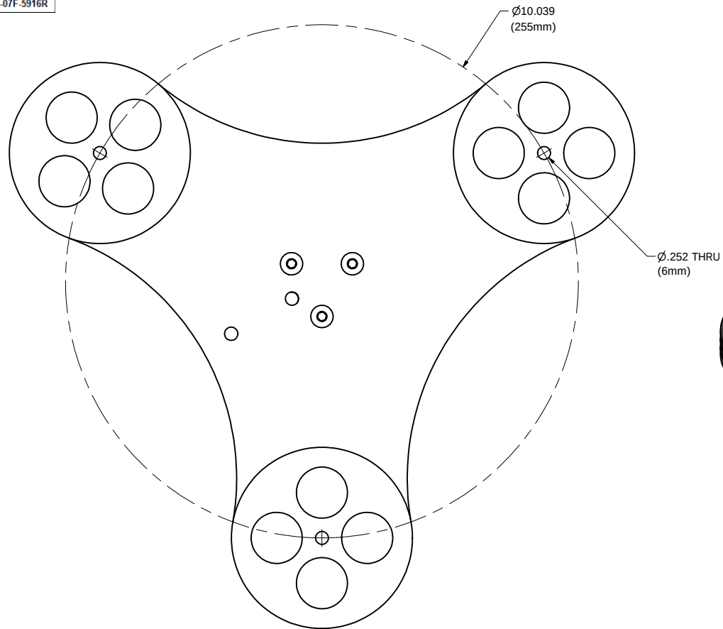
OVERHEAD VIEW AS PLATE SITS ON MAST
