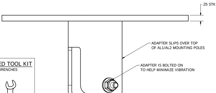
OVERHEAD VIEW
