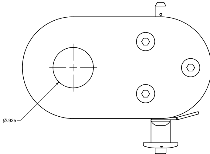
OVERHEAD VIEW
