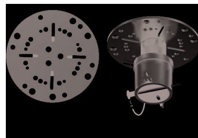
Pan & Tilt for Quickset QPT & FLIR BSM3-A-M460-MPP-00A
