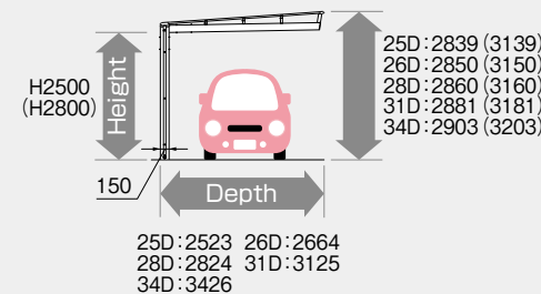
Reverse Incline Roof
