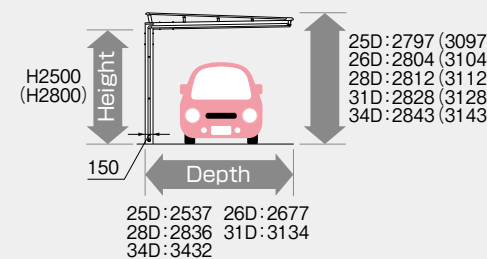
Reverse Incline Roof
