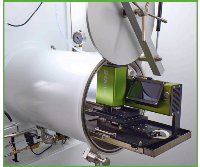
All modules fit through the glovebox antechamber
