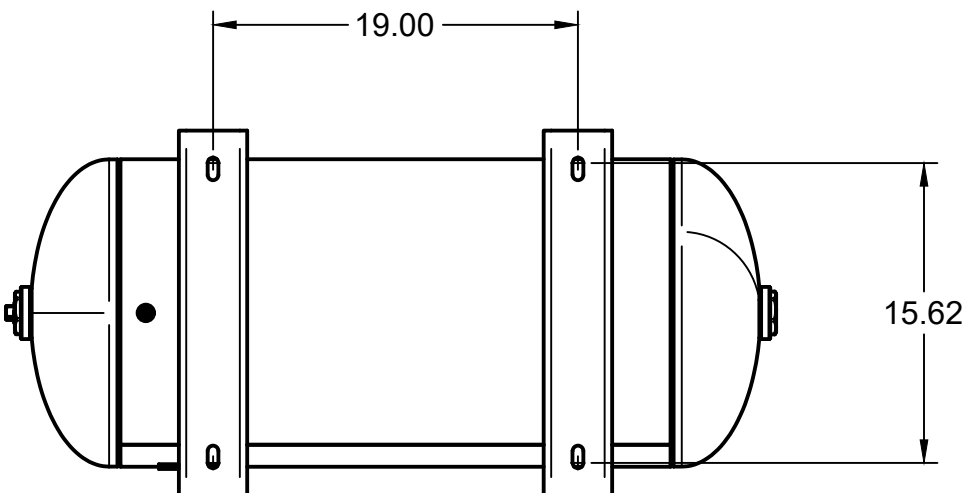
BOTTOM VIEW
