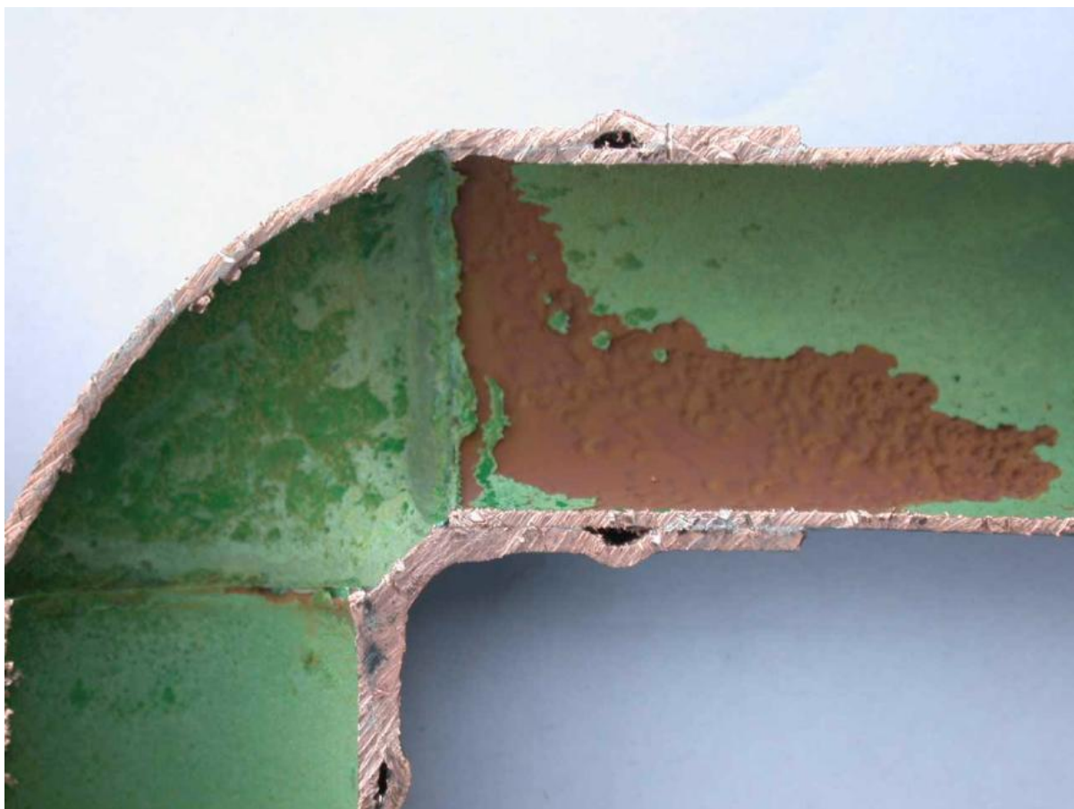
Figure 4 Erosion Corrosion at elbow.
