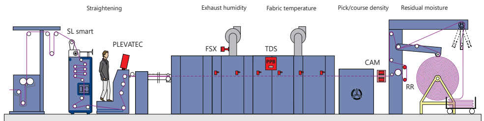
PLEVATEC smart and PLEVA sensors on a stenter frame
