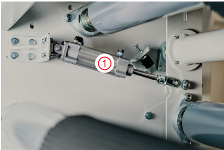
Pneumatic swing-mechanism
