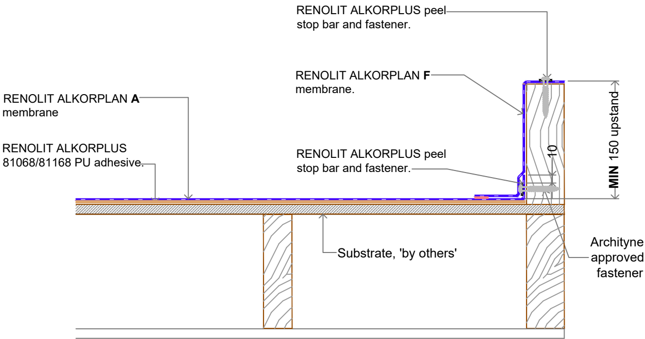
ALTERNATE VERSION WITH PEEL STOP BAR.
