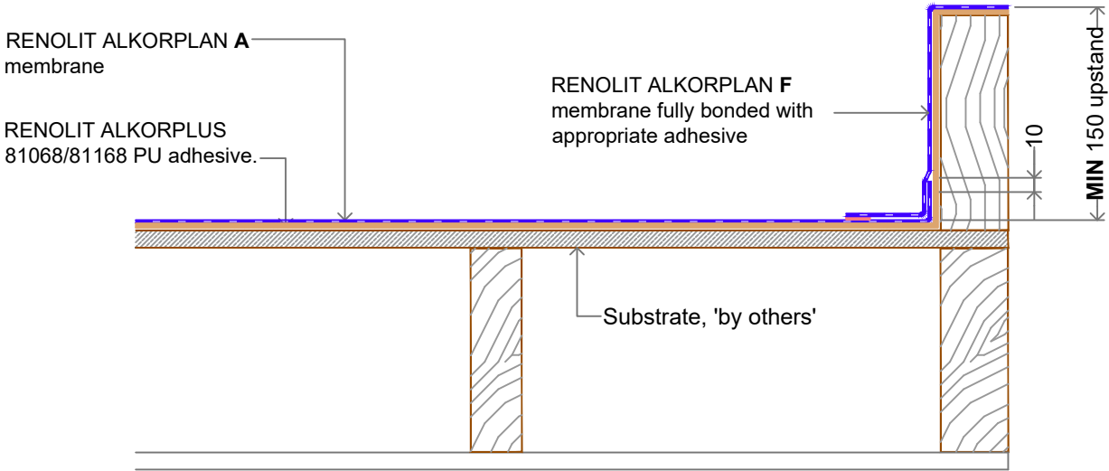
ALTERNATE VERSION FULLY BONDED UPSTAND.
