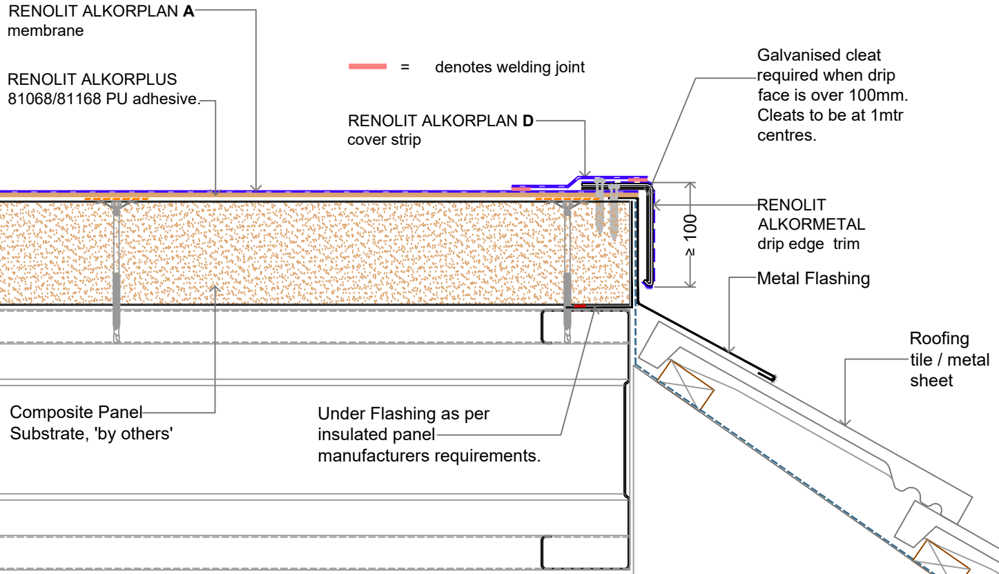
DETAIL WITH GALVANISED CLEATS
