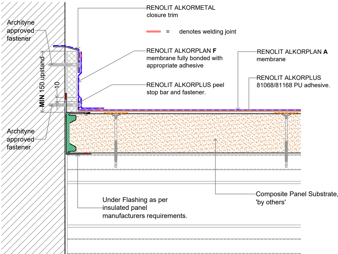
ALTERNATE VERSION WITH BAR RESTRAINT.
