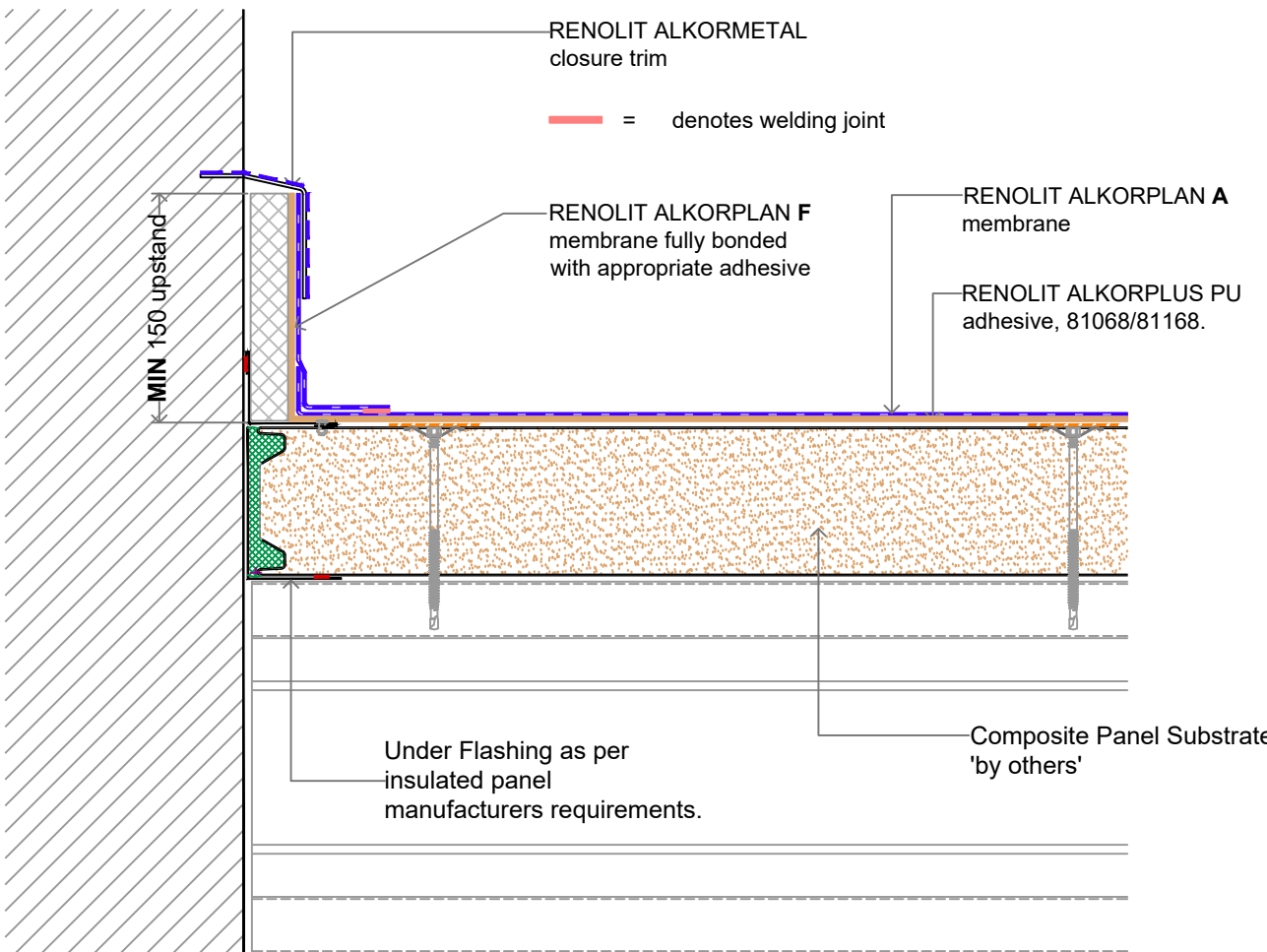
ALTERNATE VERSION FULLY BONDED UPSTAND.
