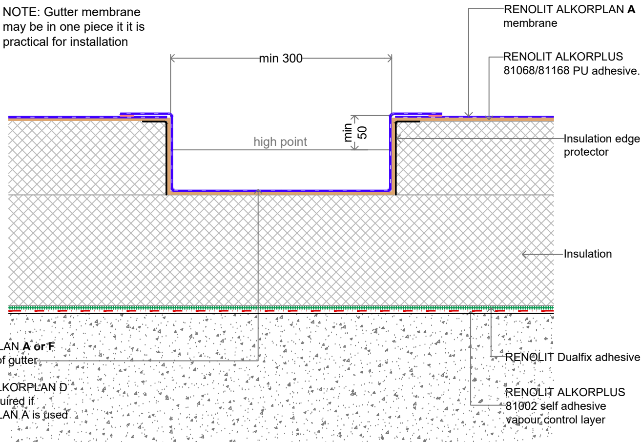
ALTERNATE VERSION FULLY BONDED.
