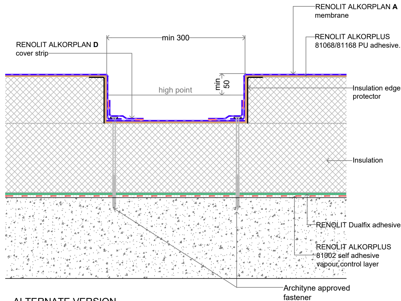
ALTERNATE VERSION WITH PEEL STOP BAR.
