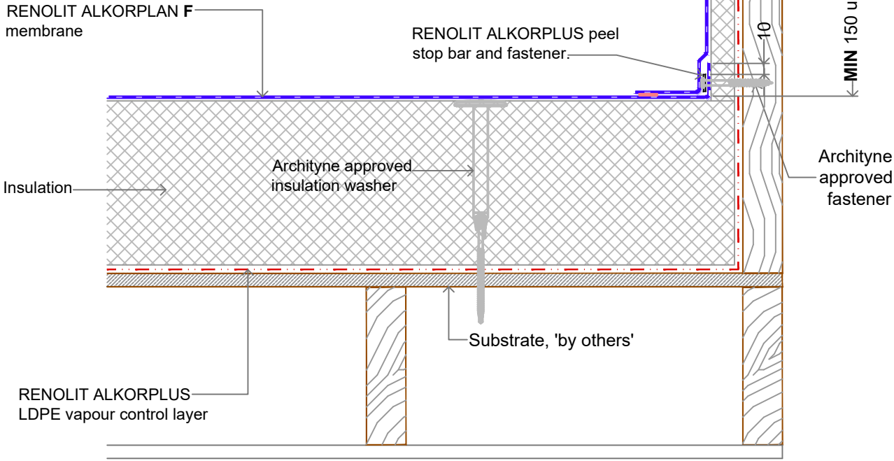
ALTERNATE VERSION WITH PEEL STOP BAR.
