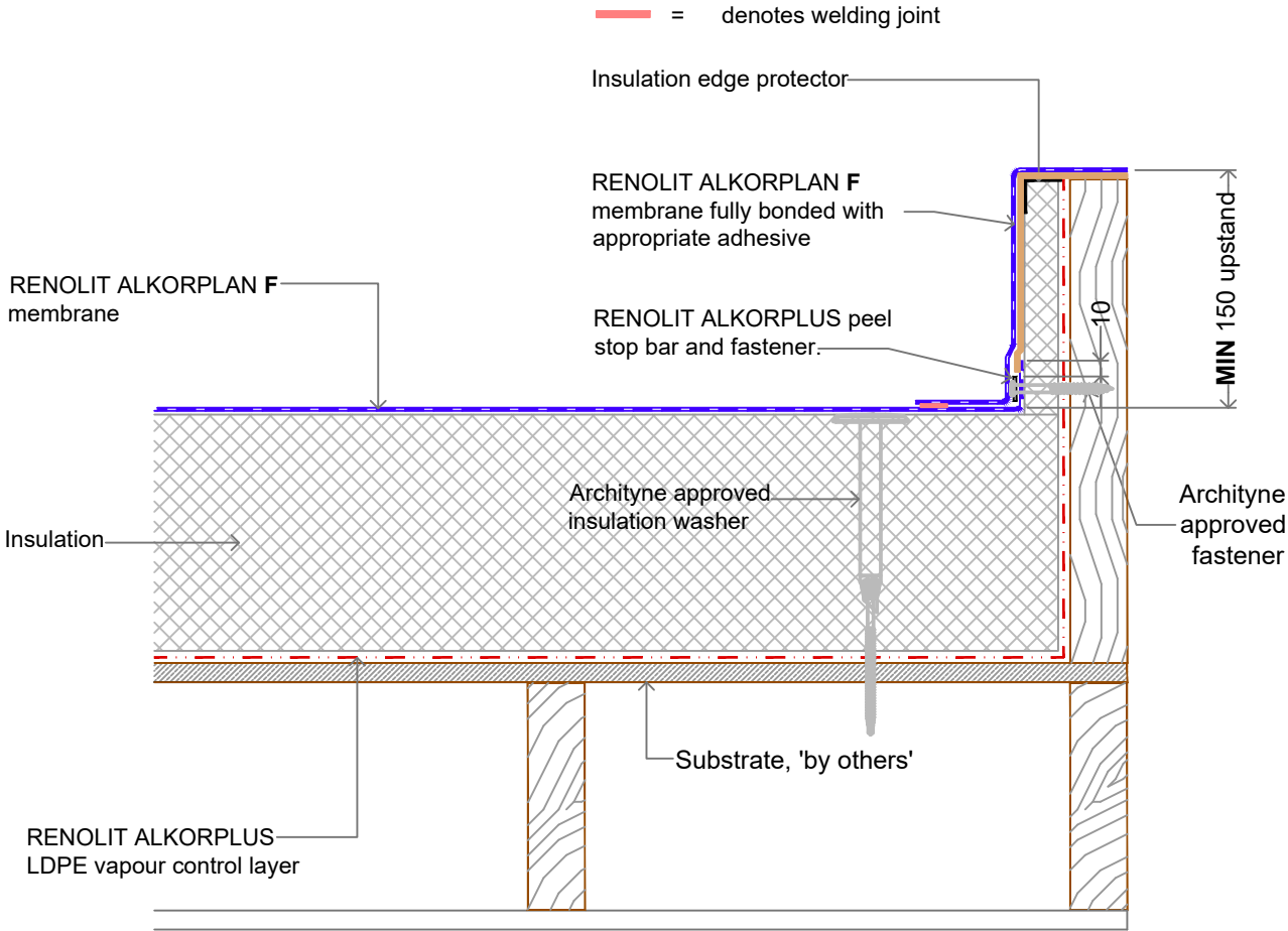
ALTERNATE VERSION FULLY BONDED UPSTAND.
